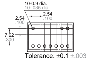
2 coil latching
