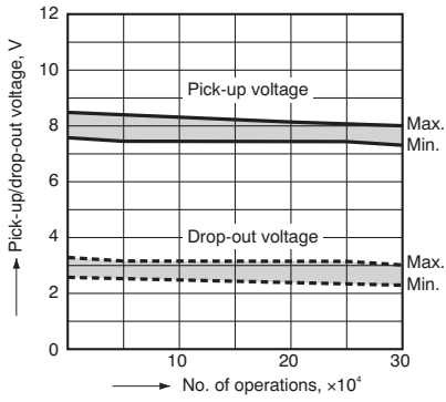
5. Electrical life test (0.01 A 24 V DC) Sample: RK1-12V; No. of samples: n = 6
