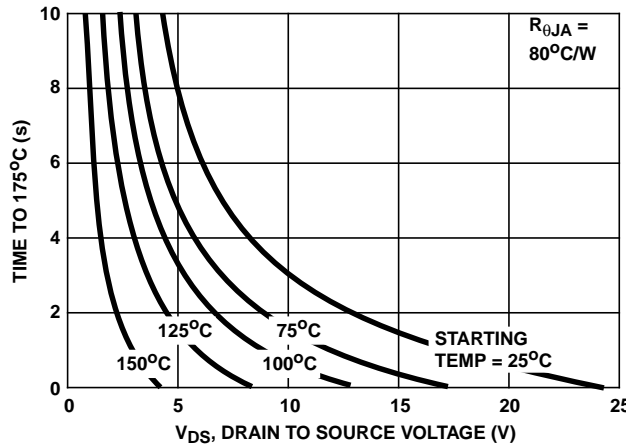
FIGURE 19. TIME TO 175°C IN CURRENT LIMITING
