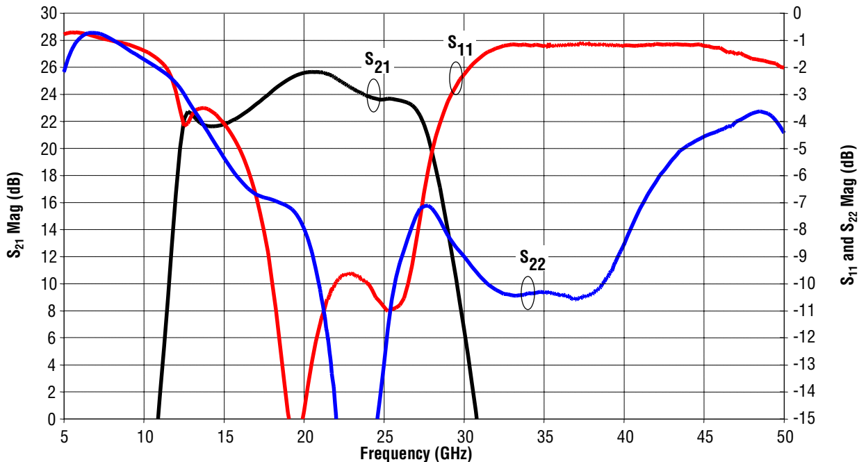
RMWL24001 Driver Amplifier Typical WideBand S-Parameters. Measurements Include 50 Ohm Test Fixture. I_{DQ} = 240 \text{ mA} V_{DD} = 4.0 \text{ V}
