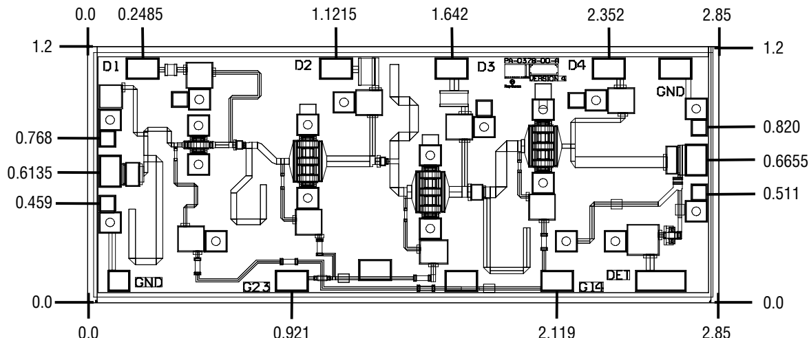
Figure 2 Chip Layout and Bond Pad Locations
