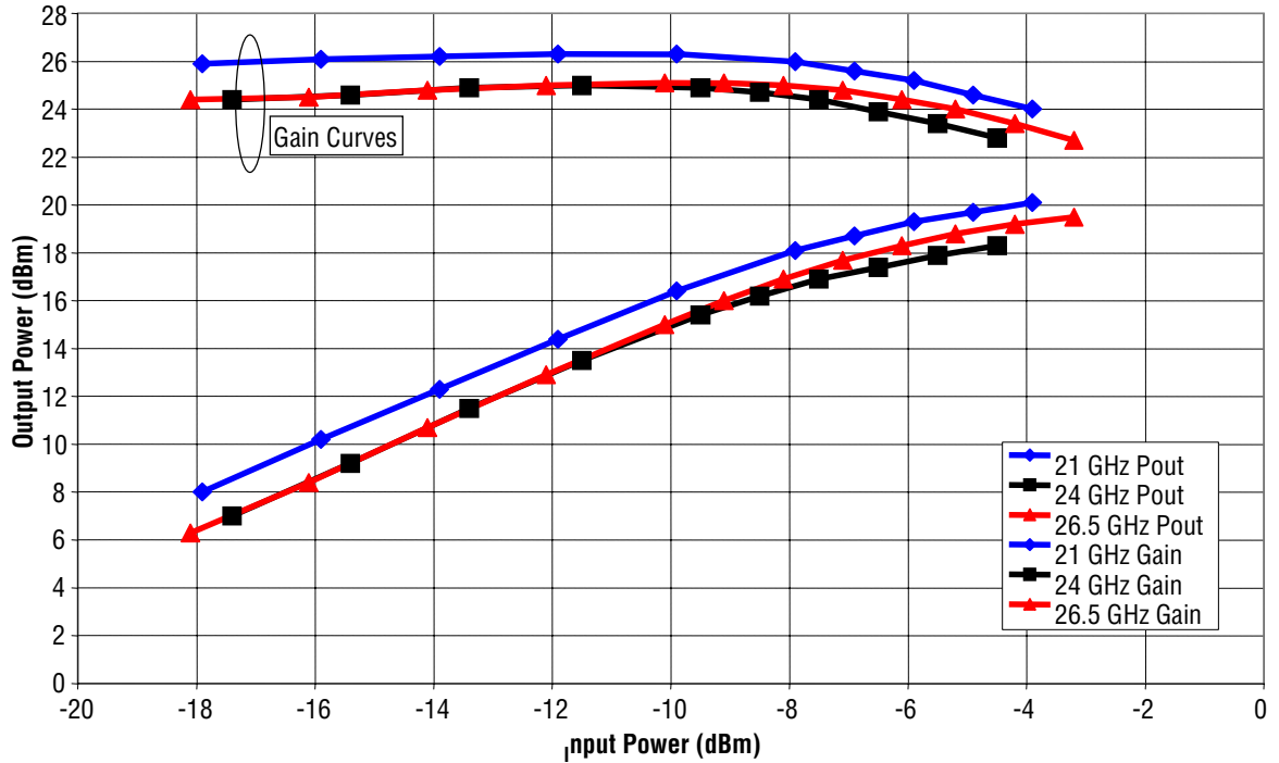
RMWL24001 Typical Power Saturation Curves. Measurements Include 50 Ohm Test Fixture. I_{DQ} = 240 \text{ mA} V_{DD} = 4.0 \text{ V}
