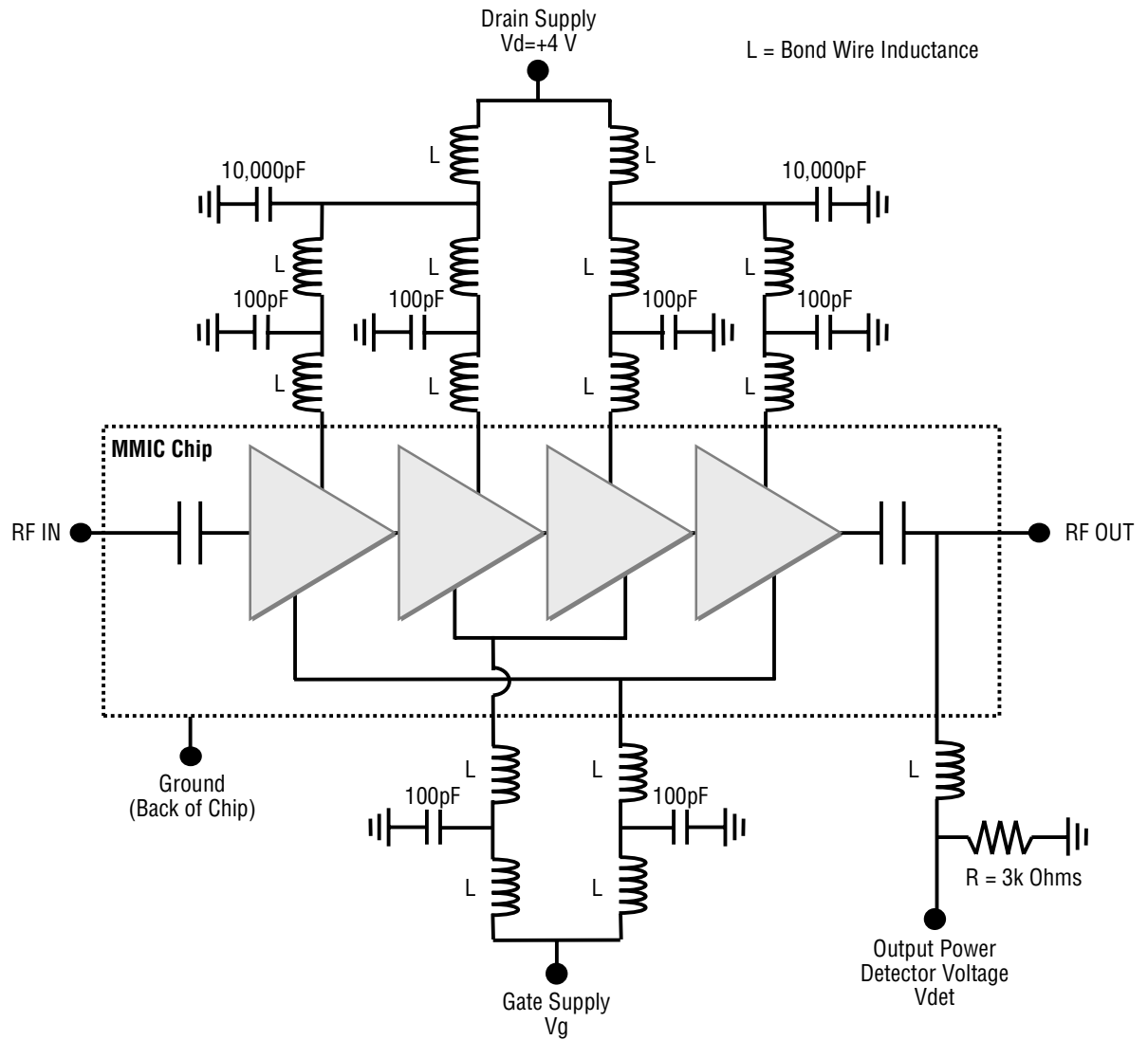
Figure 3 Recommended Application Schematic Circuit Diagram
