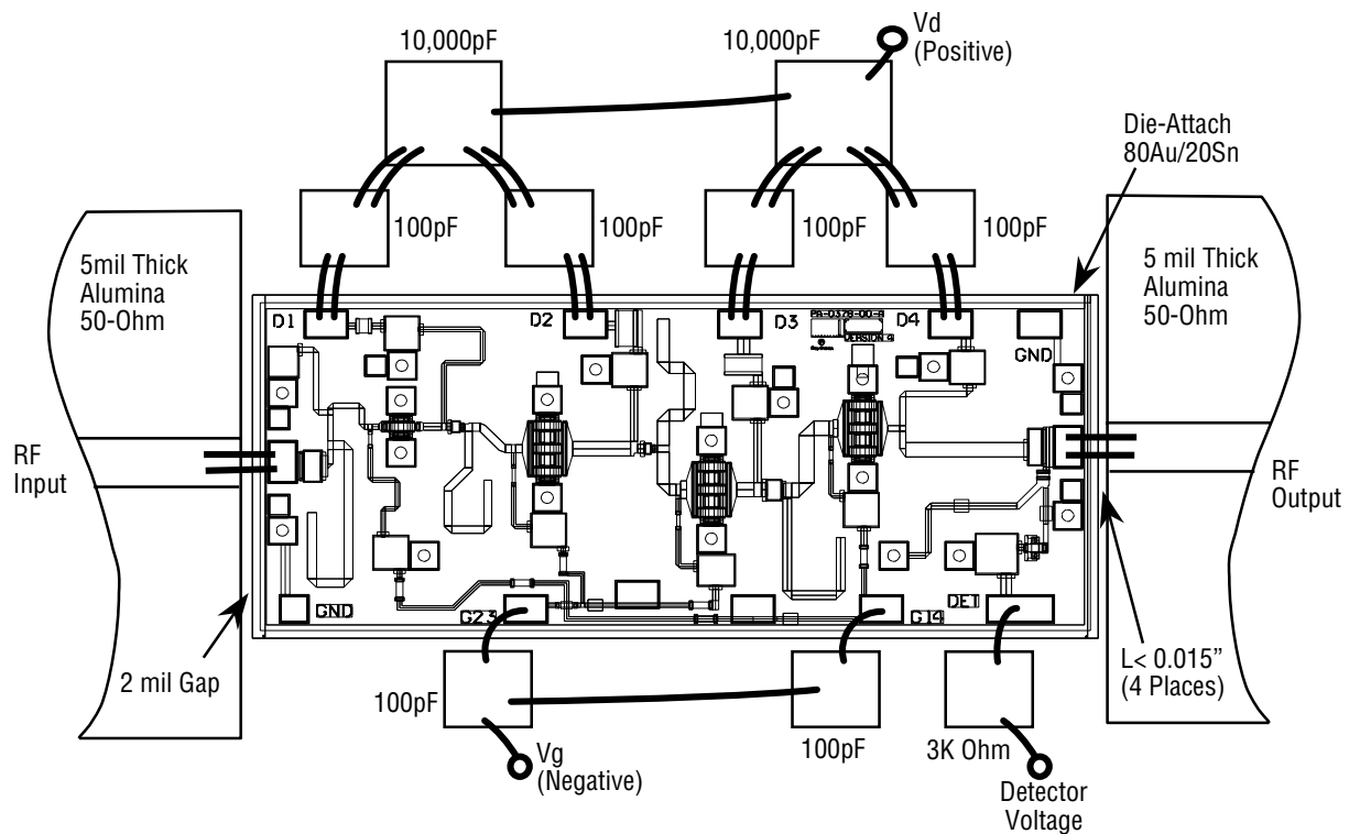
Figure 4 Recommended Assembly Diagram
