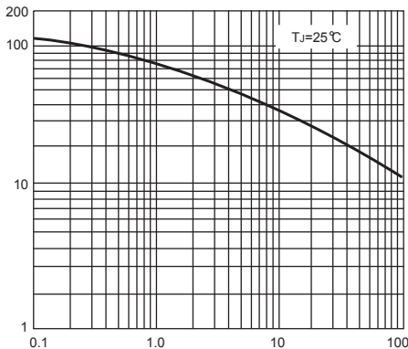
FIG. 5-TYPICAL JUNCTION CAPACITANCE
