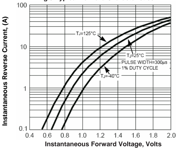
Fig.3-Typical Forward Characteristics
