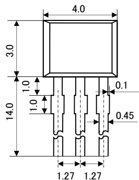
RT1N141S
