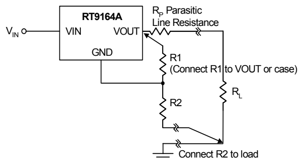
Figure 5. Best Load Regulation Using Adjustable Output Regulator
