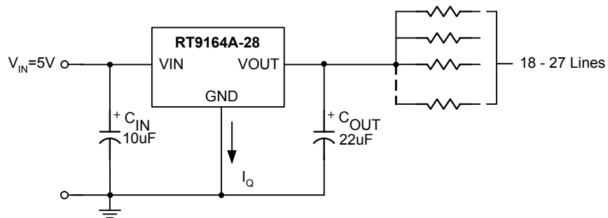
Figure 3. Fixed Voltage Regulator
