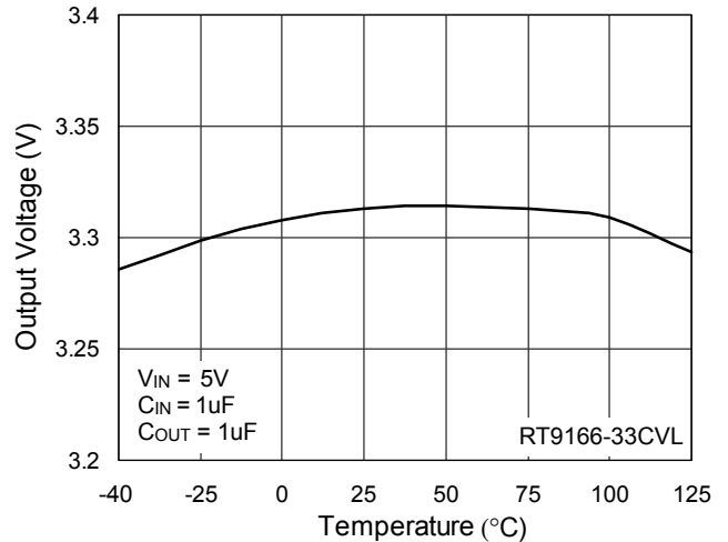
Temperature Stability
