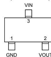
SOT-23-3 (L-Type) (RT9166)
