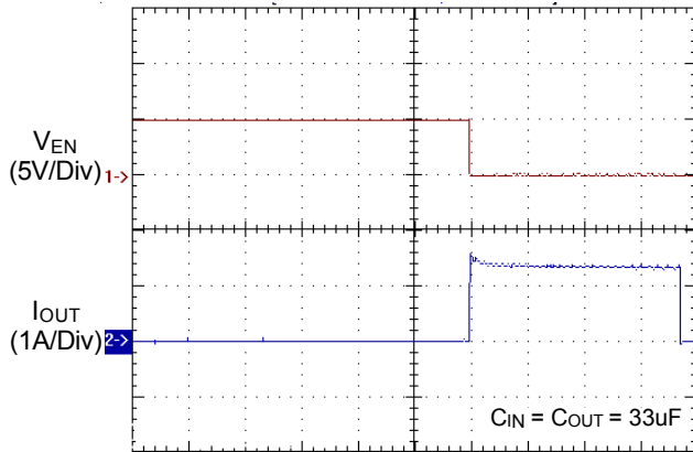
Short Circuit Current Response
