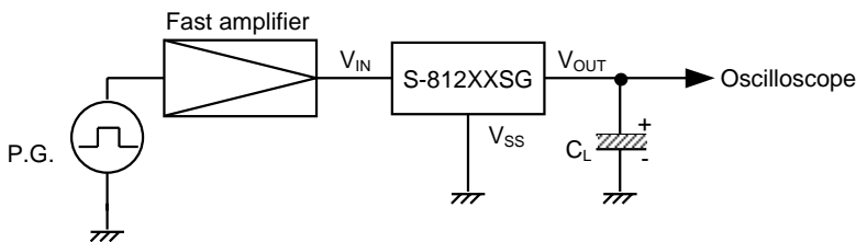
Figure 8 Measuring circuit
