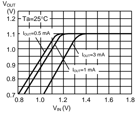
1.3 S-81220SG series
