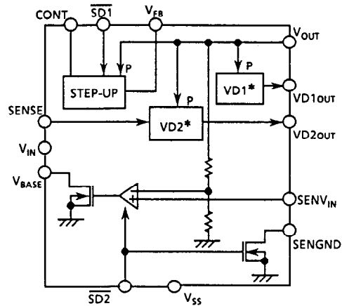
(2) S-8311 Series
