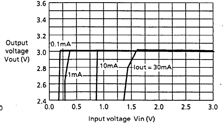
(b) Input voltage – Output voltage characteristics
