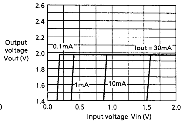
(b) Input voltage – Output voltage characteristics (fall in input voltage)
