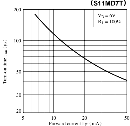
Fig.11-a Turn-on Time vs. Forward Current
