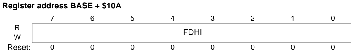
Figure 3-12 8-bit Flash Data High Register (FDATAHI)
