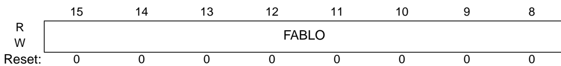
Figure 3-11 Flash 8-bit Address Low Register (FADDRLO)
