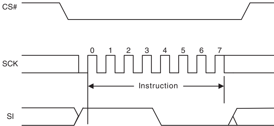
Figure 9.60 Software Reset Command Sequence
