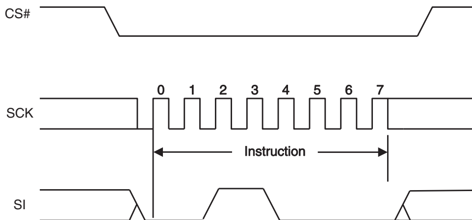
Figure 9.16 Clear Status Register (CLS) Command Sequence
