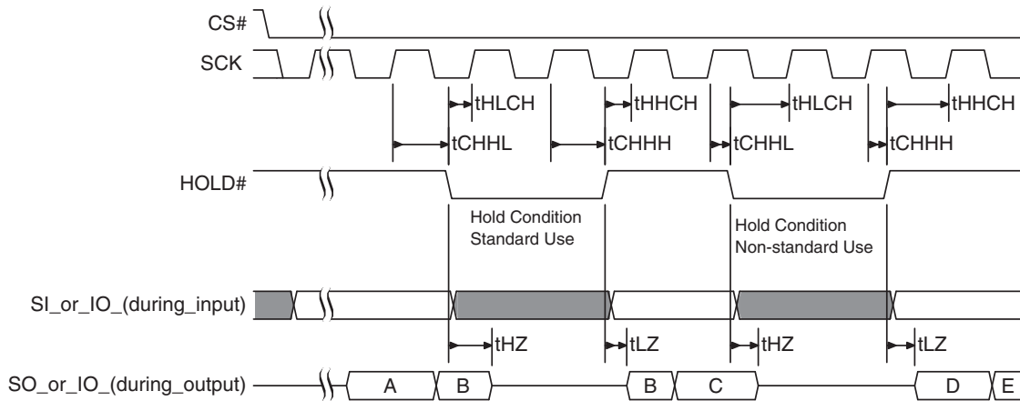
Figure 5.14 Hold Timing
