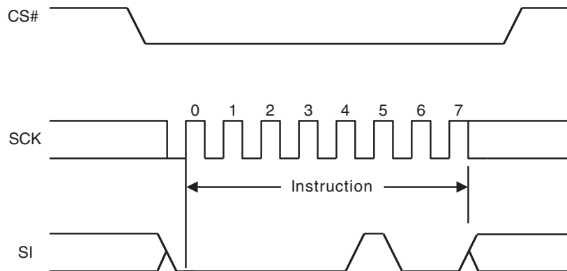
Figure 9.15 Write Disable (WRDI) Command Sequence
