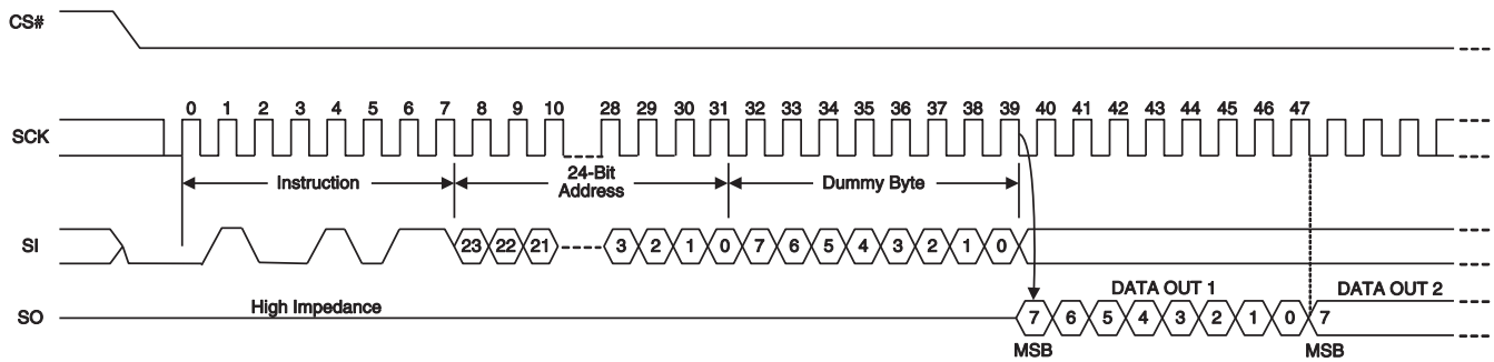
Figure 9.47 OTP Read Command Sequence
