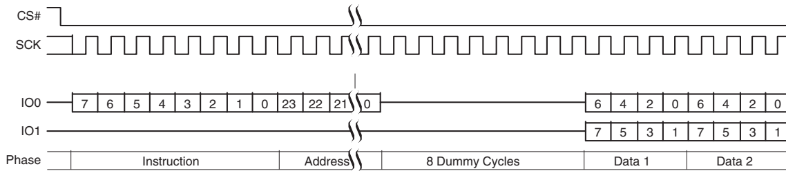
Figure 9.24 Dual Output Read Command Sequence (3-Byte Address, 3Bh [ExtAdd=0], LC=10b)
