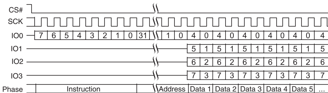
Figure 3.8 Quad Output Command without Latency
