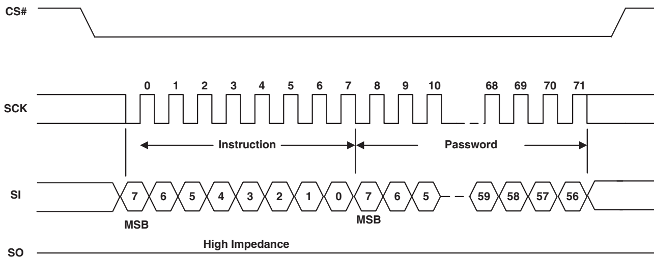
Figure 9.58 Password Program Command Sequence
