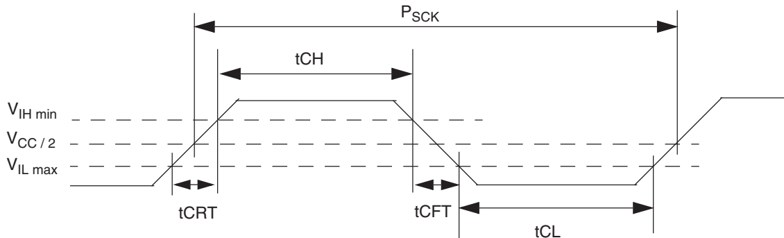
Figure 5.10 Clock Timing
