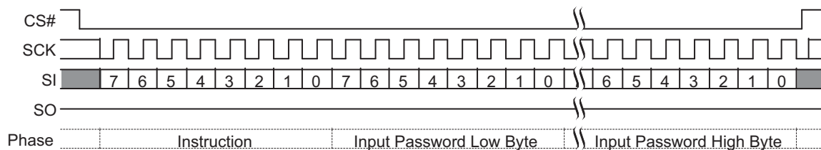
Figure 9.66 Password Unlock Command Sequence
