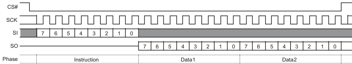
Figure 3.5 Single Bit Wide Output Command
