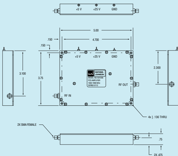
OUTLINE DRAWING
