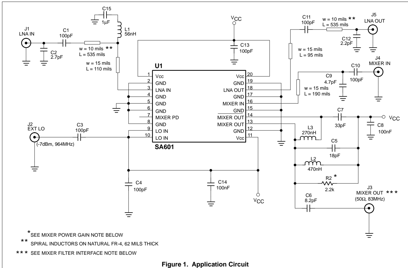
Figure 1. Application Circuit
