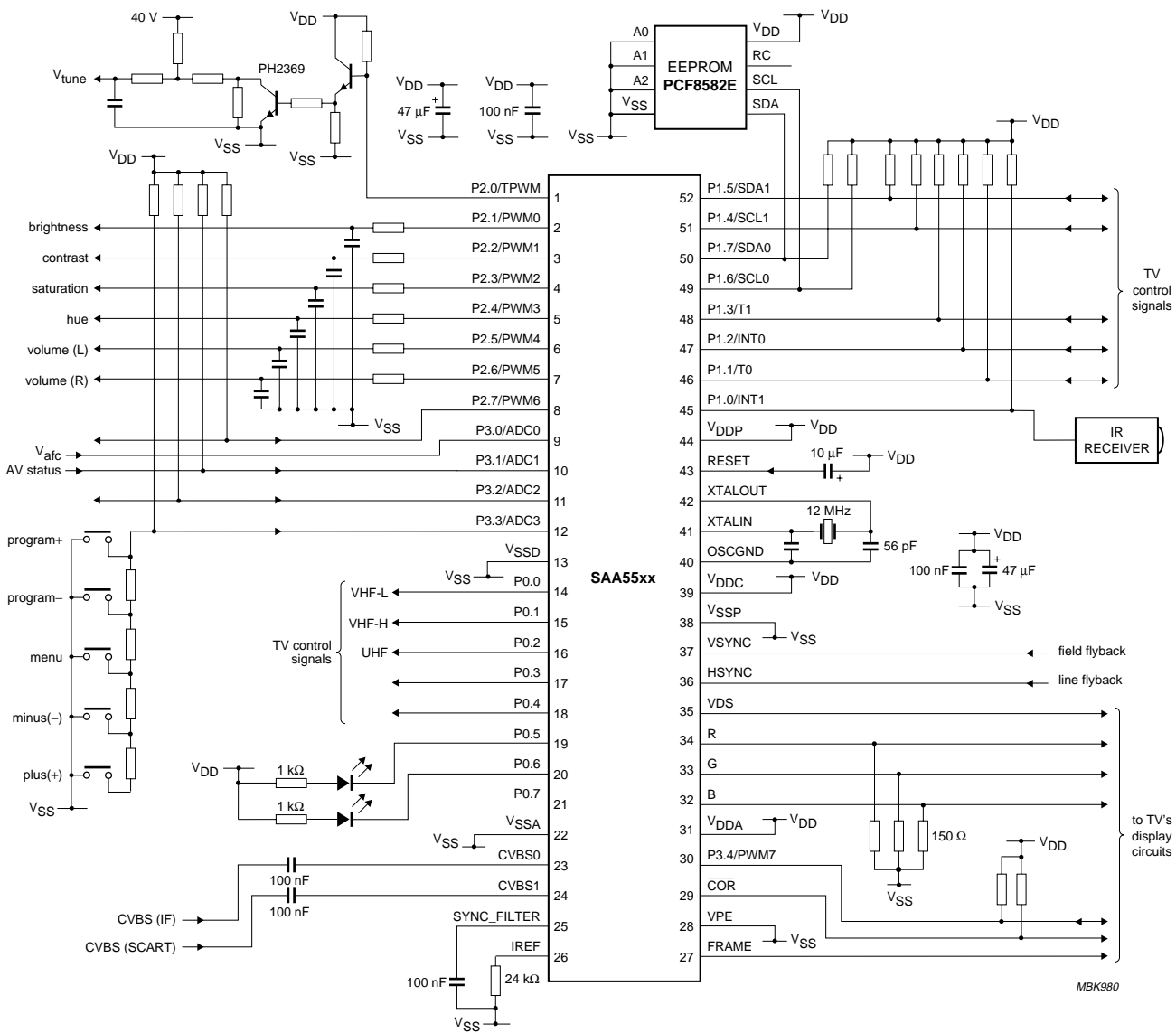
Fig.29 Application diagram.
