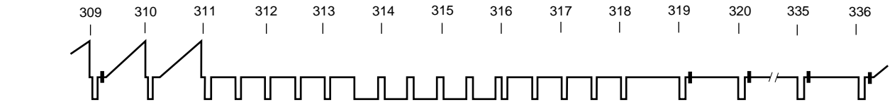
(b) 4th field CVBS output signal
