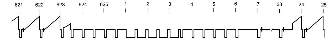
(a) 3rd field CVBS output signal
