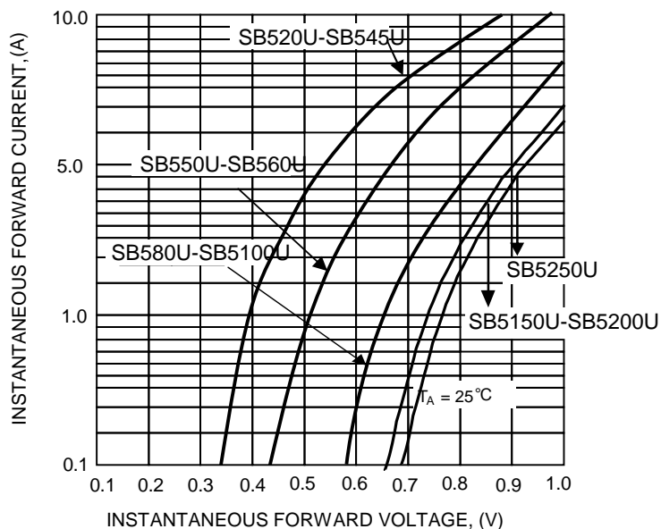
FIG.2-TYPICAL FORWARD CHARACTERISTICS
