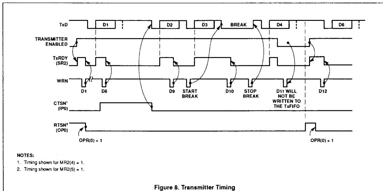
Figure 8. Transmitter Timing
