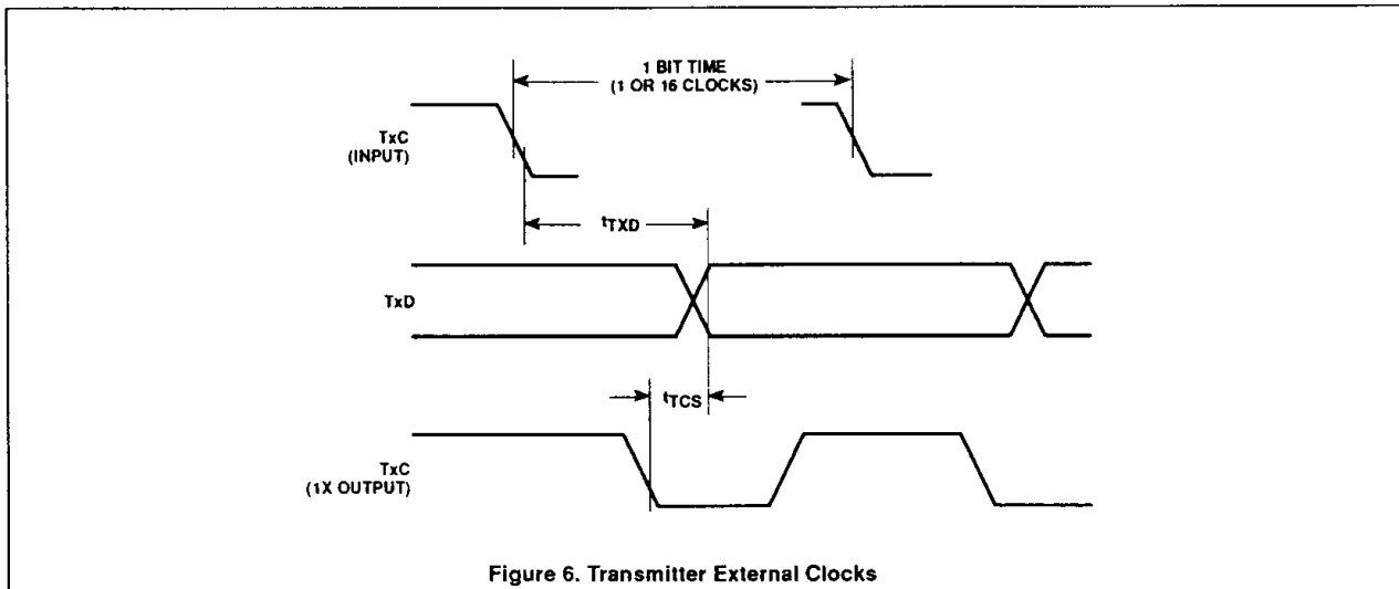
Figure 6. Transmitter External Clocks
