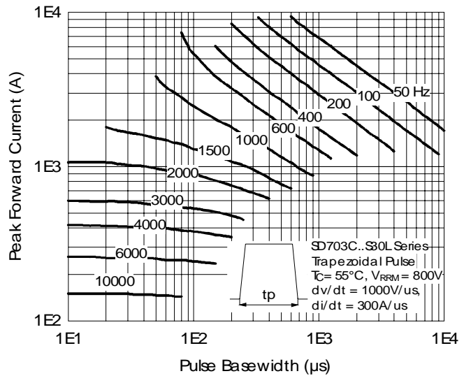
Fig. 37 - Frequency Characteristics
