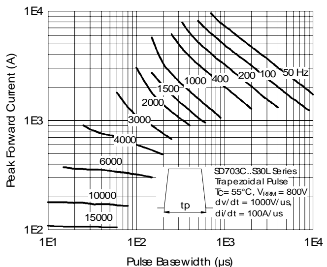
Fig. 39 - Frequency Characteristics
