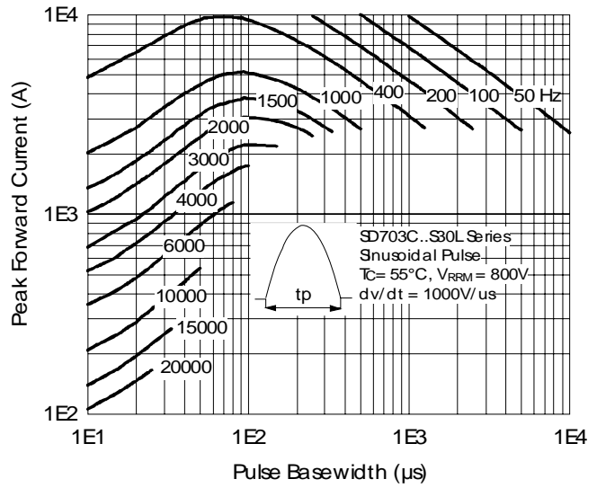
Fig. 35 - Frequency Characteristics
