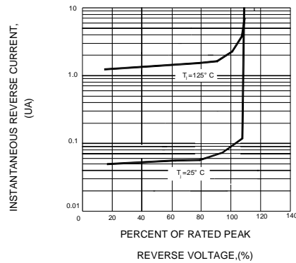
FIG.4-TYPICAL REVERSE CHARACTERISTICS
