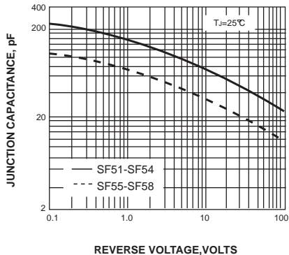
FIG. 5-TYPICAL JUNCTION CAPACITANCE
