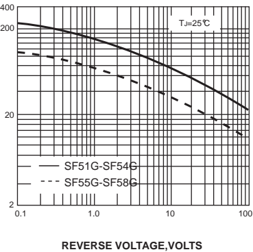
FIG. 5-TYPICAL JUNCTION CAPACITANCE
