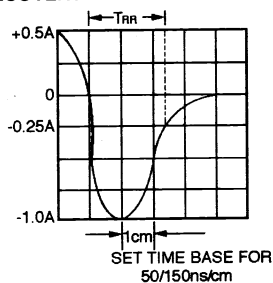
FIG. 5-TEST CIRCUIT DIAGRAM AND REVERSE RECOVERY TIME CHARACTERISTICS
