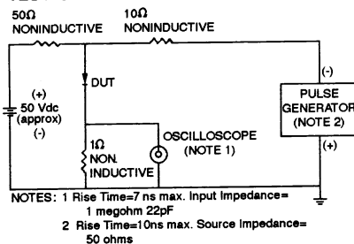
FIG. 5-TEST CIRCUIT DIAGRAM AND REVERSE RECOVERY TIME CHARACTERISTICS
