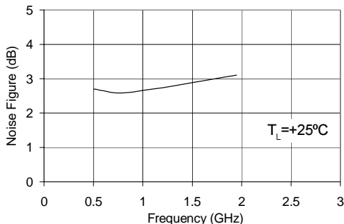
Noise Figure vs. Frequency V_D = 2.6\text{ V} , I_D = 20\text{ mA}
