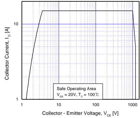
Fig 16. Turn-Off SOA
