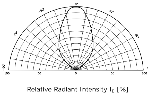
Fig. 5 Radiation Diagram
