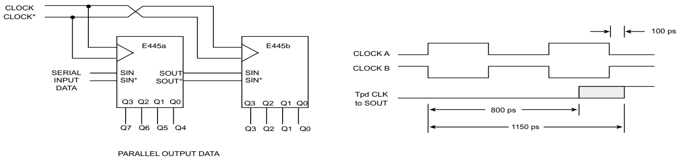
Figure 4. Extended Frequency 1:8 Demultiplexer
