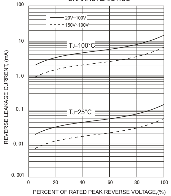
FIG.4-TYPICAL REVERSE CHARACTERISTICS
