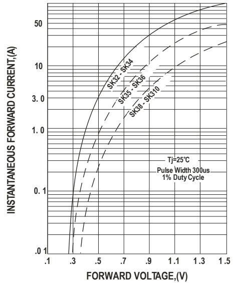
FIG.2-TYPICAL FORWARD CHARACTERISTICS
