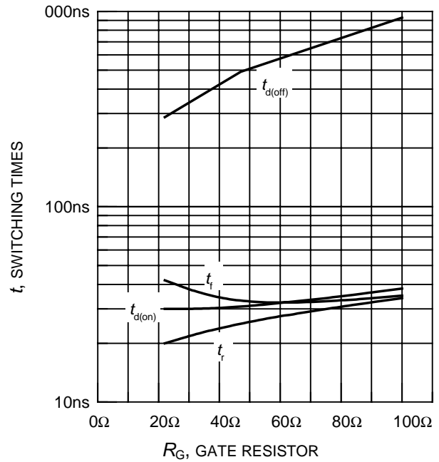
Figure 10. Typical switching times as a function of gate resistor (inductive load, T_j = 150^{\circ}\text{C} , V_{\text{CE}} = 800\text{V} , V_{\text{GE}} = +15\text{V}/0\text{V} , I_C = 8\text{A} , dynamic test circuit in Fig.E )
