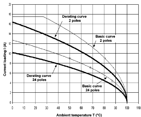
BL 3.5/SL-SMT 3.5/90°, 2 and 24 poles Conductor H07V-K1.5mm 2
