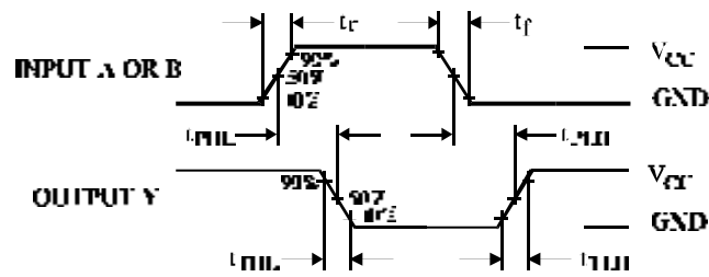
Figure 2. Switching Waveforms
