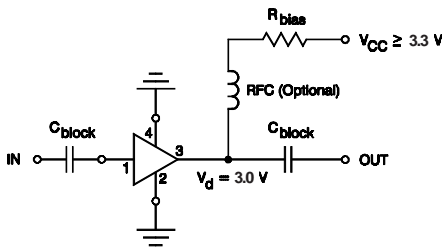
Typical Biasing Configuration
