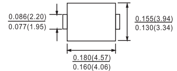
DO-214AA(SMB)
