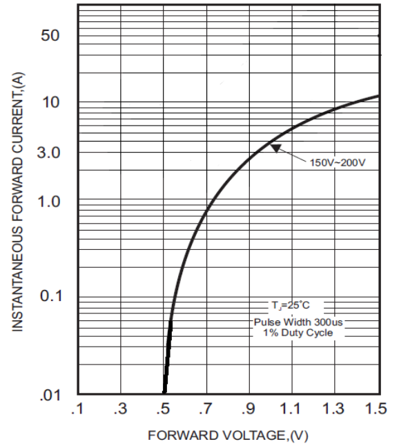
FIG.2-TYPICAL FORWARD CHARACTERISTICS
