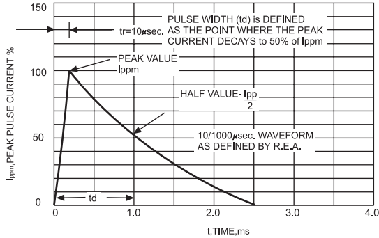
FIG.3-PULSE WAVEFORM
