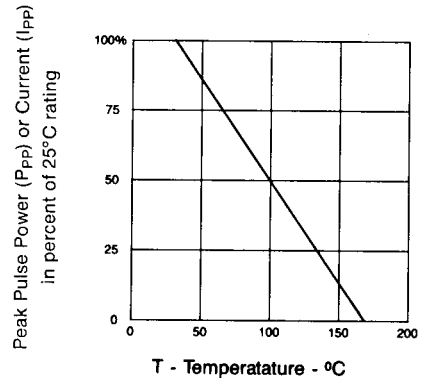
FIGURE 3 DERATING CURVE
