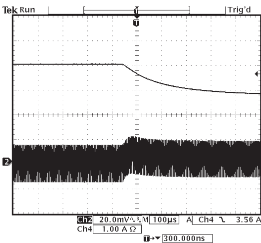
Figure 5: Typical Transient Response 75% - 50% Step Load Change (Channel 2: V_o , Channel 4: I_o )
