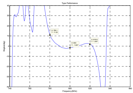
Phase Linearity(f0±20MHz)
