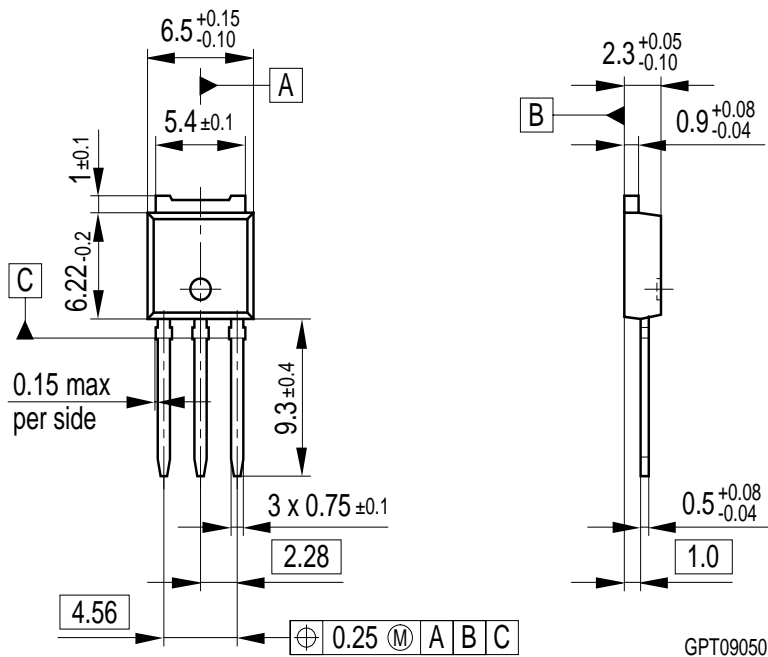
P-TO-251-3-1 (I-PAK)
