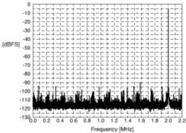
FFT Plot
