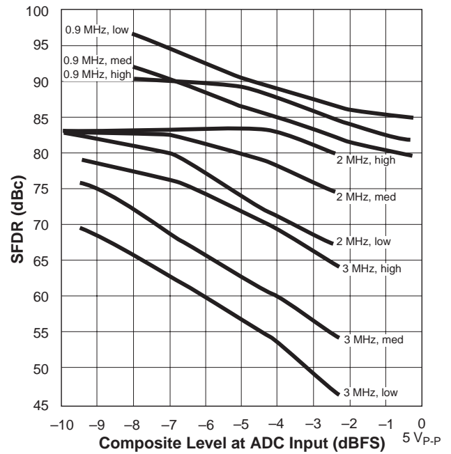
Spurious Free Dynamic Range
