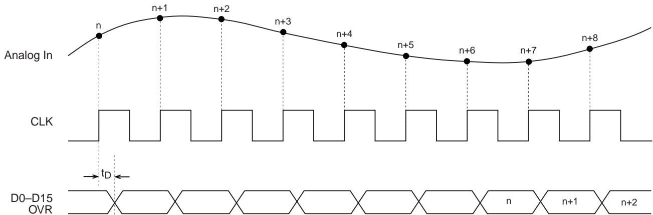
Figure 3 – Timing Diagram 1
