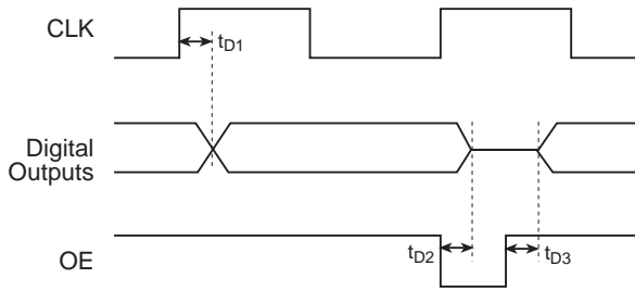
Figure 5 – Timing Diagram 2
