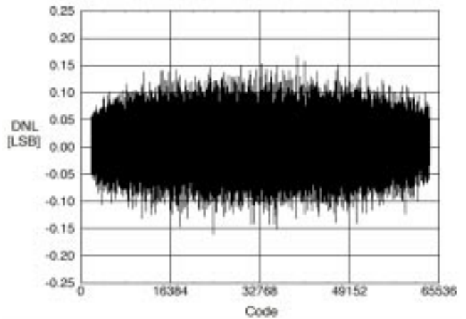
Typical Differential Non-Linearity (DNL)
