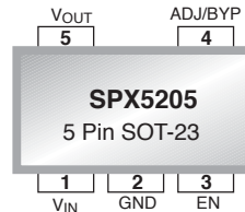
Adjustable Output Voltage
