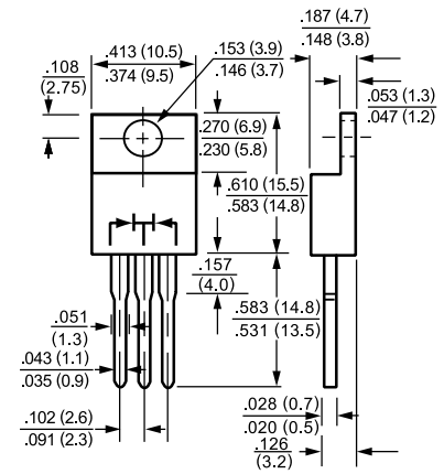
TO-220
