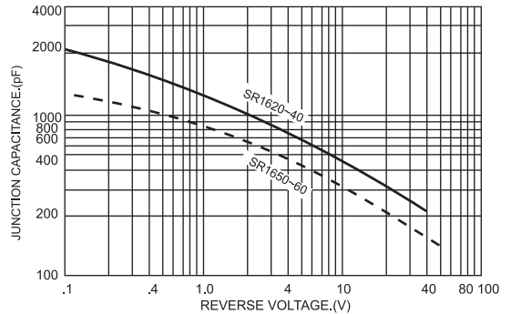
FIG.4-TYPICAL JUNCTION CAPACITANCE
