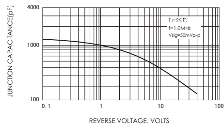
FIG.5-TYPICAL JUNCTION CAPACITANCE
