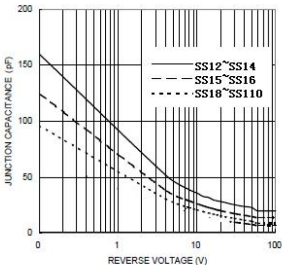
FIG. 5-TYPICAL JUNCTION CAPACITANCE
